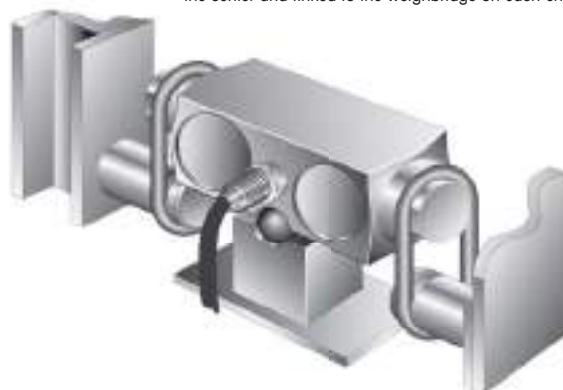
Double-ended shear beam load cells are supported in the center and linked to the weighbridge on each end.
