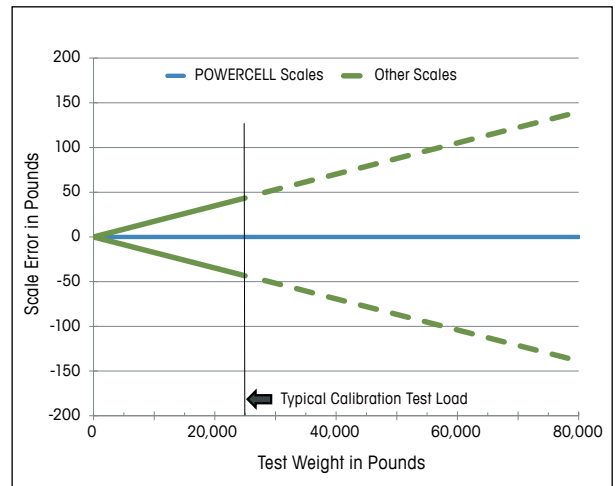
Accuracy Comparison POWERCELL® vs. Analog Load Scales
